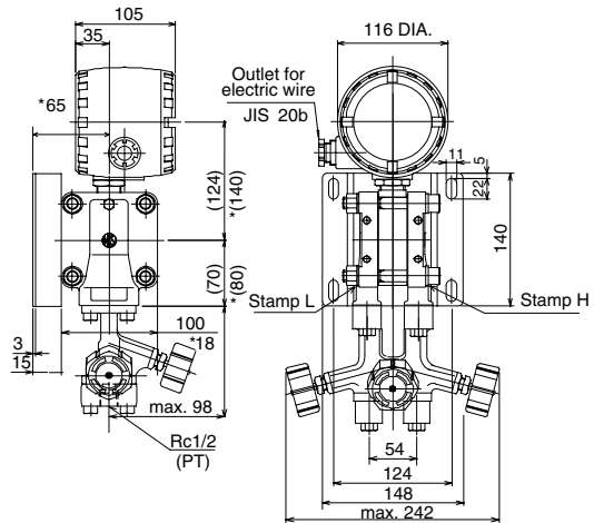
Surface mounting 3-way manifold valve
