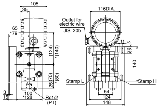
Surface mounting
