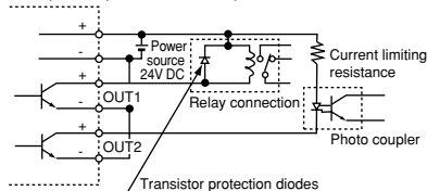
Example of open collector output
